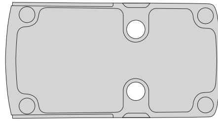
THE DOCTER FOOTPRINT (BURRIS FASTFIRE 3)
