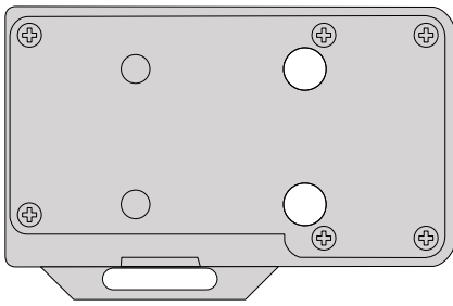
THE C-MORE FOOTPRINT (VORTEX RAZOR)
