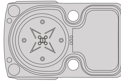
THE RMR FOOTPRINT (TRIJICON RMR TYPE 2)
